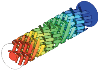
Static mixer simulation in ANSYS fluid dynamics software
