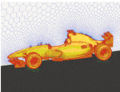
Polyhedral mesh of a race car as used with ANSYS FLUENT software. The use of polyhedral meshes speeds up many simulations.
