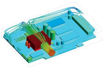
A conjugate heat-transfer solution and subsequent thermal-stress analysis of a computer graphics card; fluid streamlines and solid temperatures (left) and thermal stresses (right) are shown for the coupled simulation
